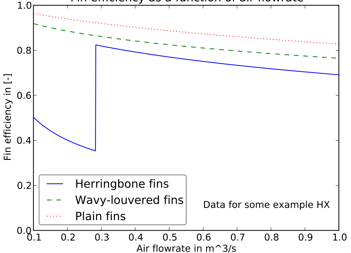
Fin efficiency as a function of air flowrate
