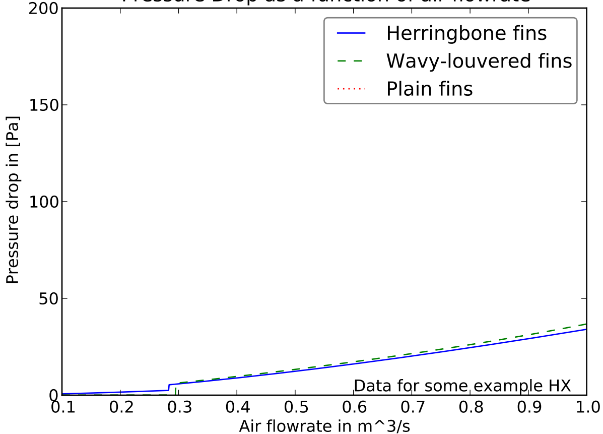
Pressure Drop as a function of air flowrate
