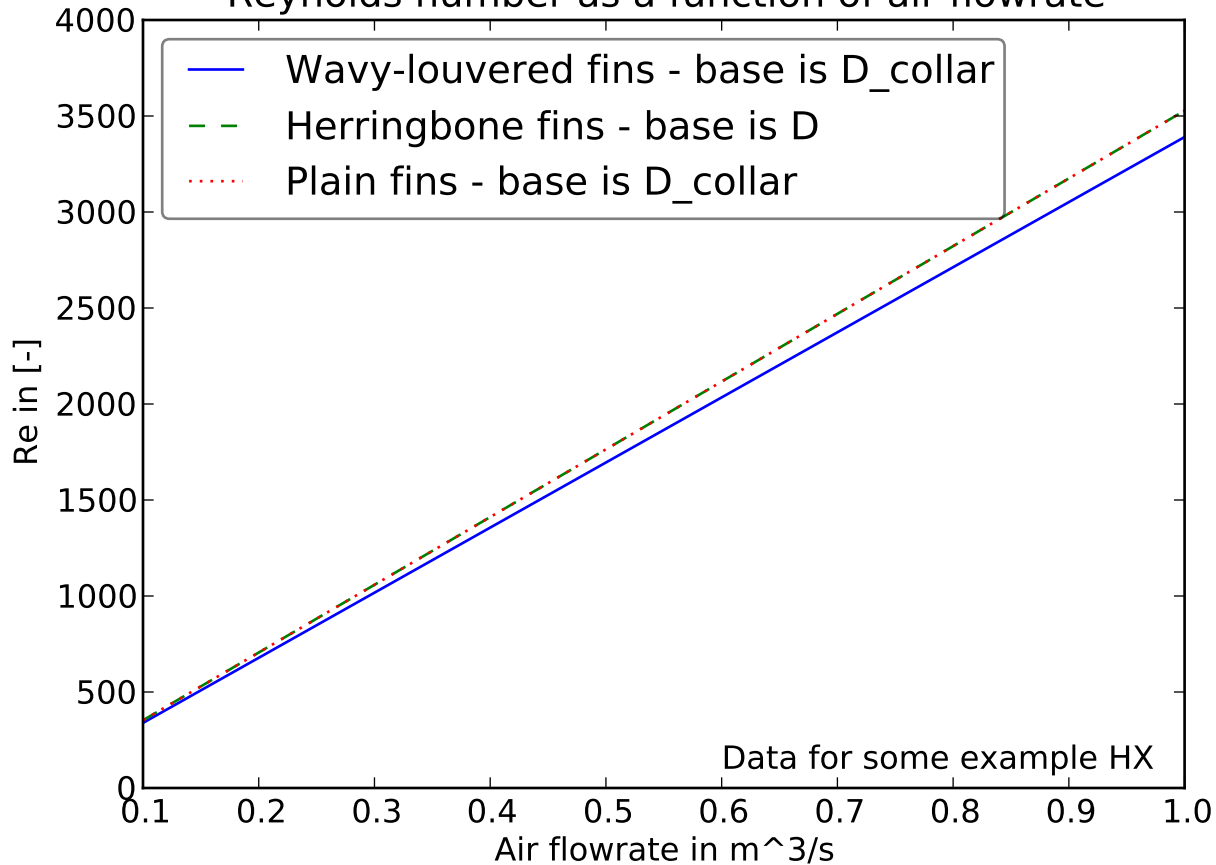
Reynolds number as a function of air flowrate
