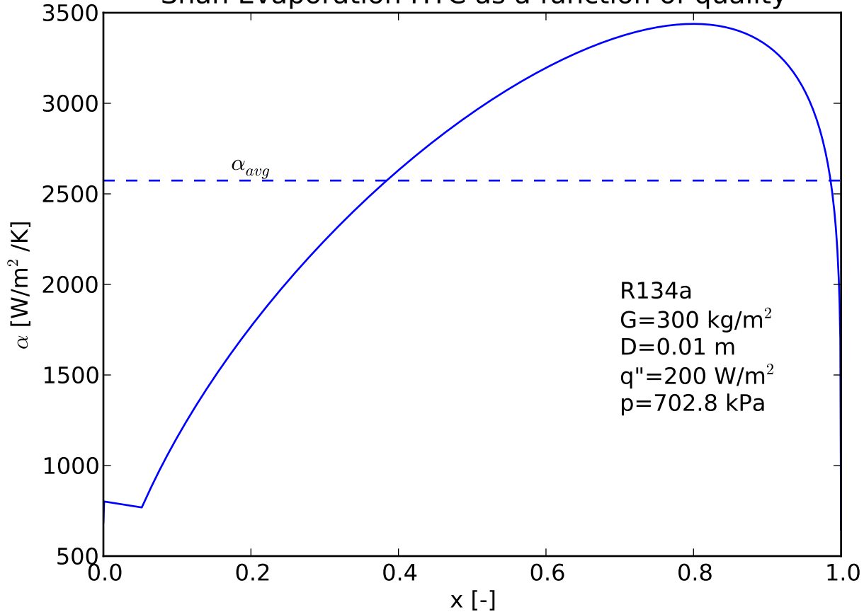
Shah Evaporation HTC as a function of quality
